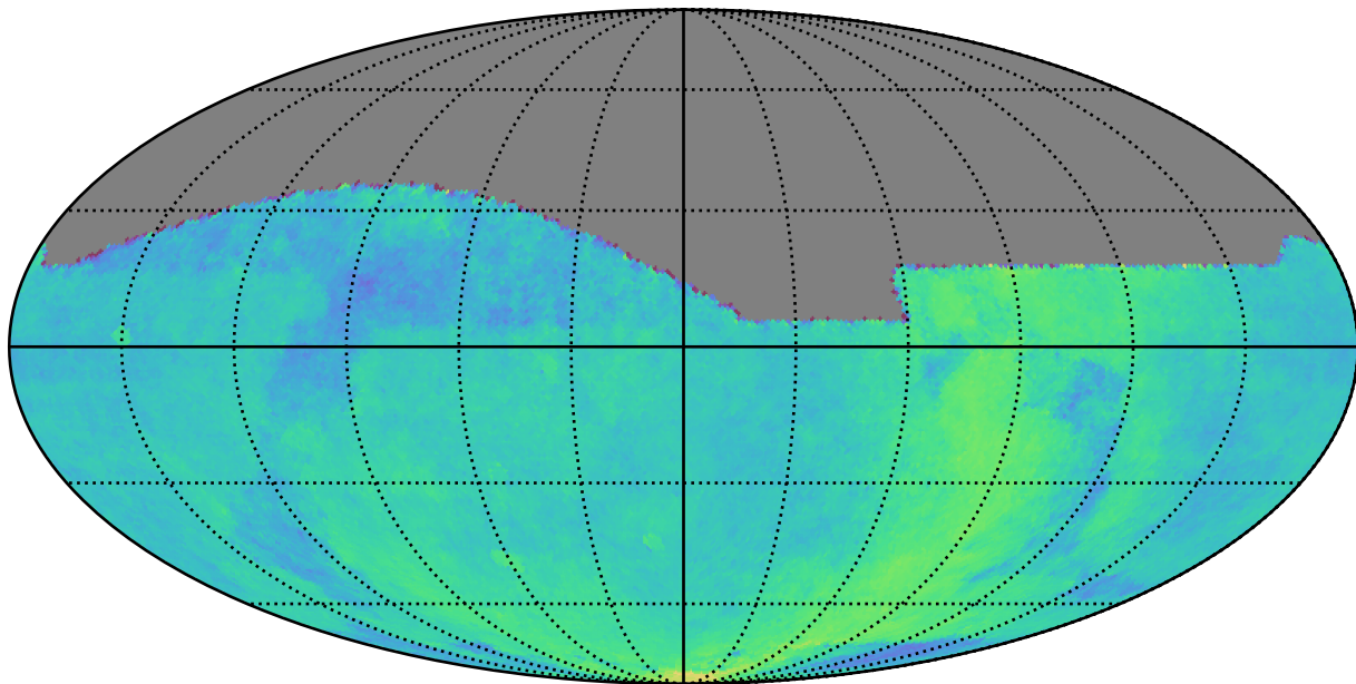
early_u_fpextra2.0_v3.4_10yrs All sky: Parallax Coverage @ 24.0
