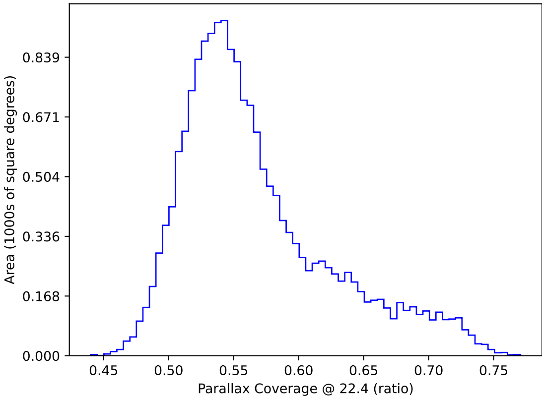
early_u_fpextra2.0_v3.4_10yrs WFD: Parallax Coverage @ 22.4
