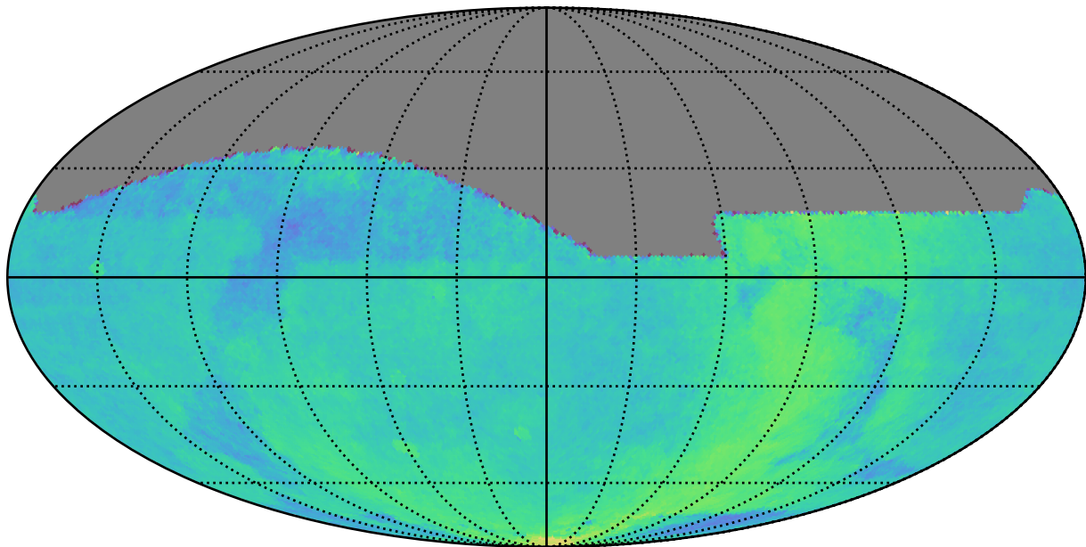
early_u_fpextra2.0_v3.4_10yrs All sky: Parallax Coverage @ 22.4
