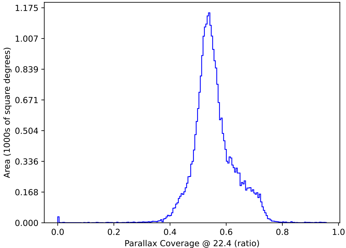
early_u_fpextra2.0_v3.4_10yrs All sky: Parallax Coverage @ 22.4
