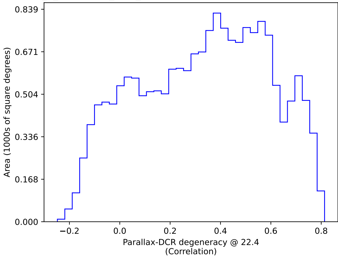
early_u_fpextra2.0_v3.4_10yrs WFD: Parallax-DCR degeneracy @ 22.4
