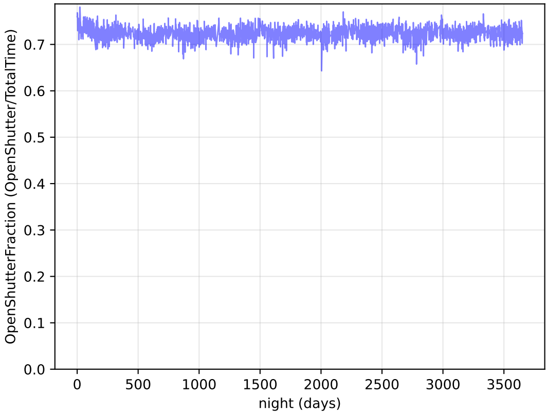
early_u_fpextra2.0_v3.4_10yrs Per night: OpenShutterFraction
