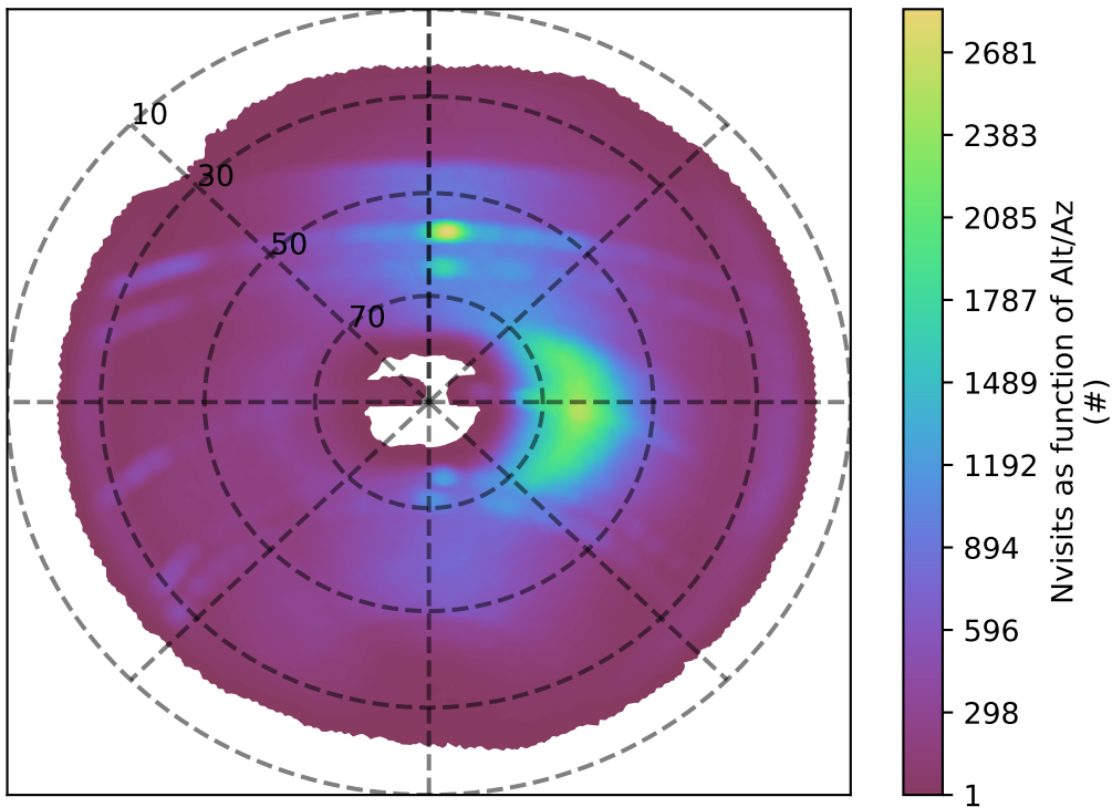
early_u_fpextra2.0_v3.4_10yrs i band: Nvisits as function of Alt/Az
