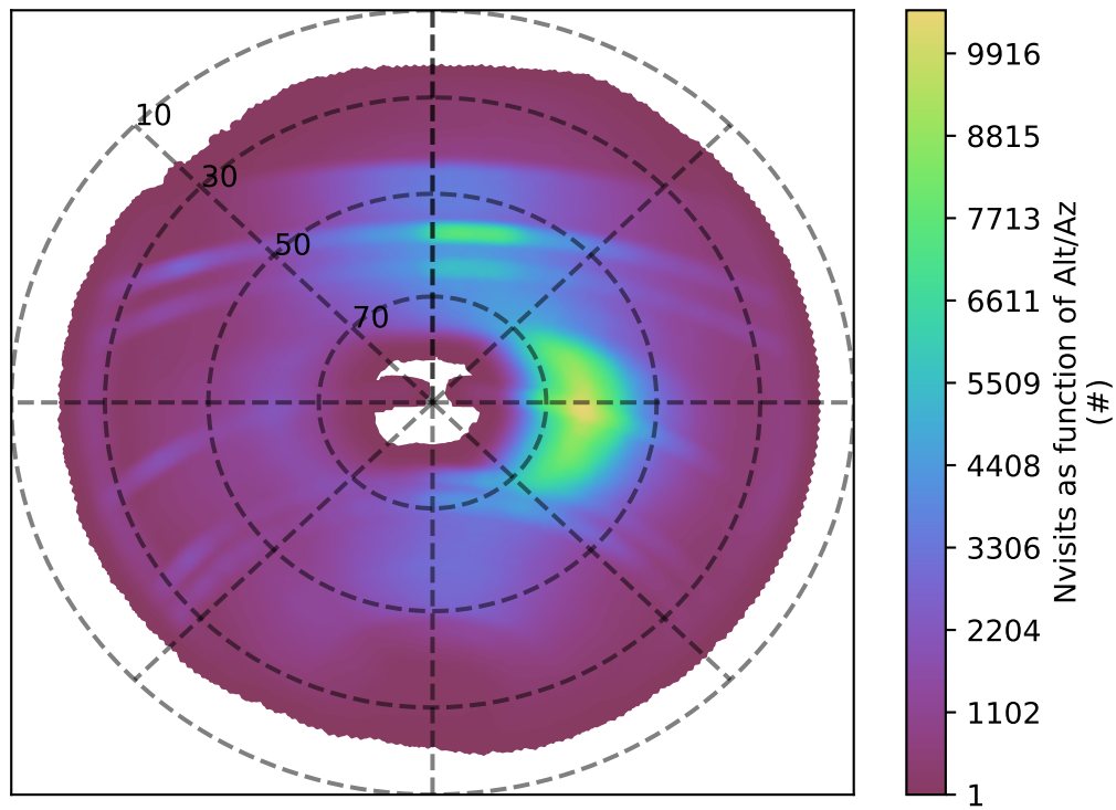
early_u_fpextra2.0_v3.4_10yrs all bands: Nvisits as function of Alt/Az
