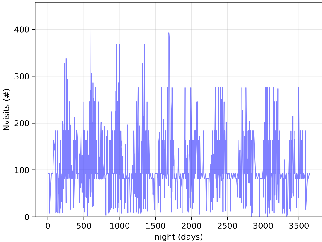
early_u_fpextra2.0_v3.4_10yrs DDF: Nvisits
