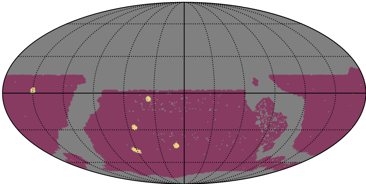
early_u_fpextra2.0_v3.4_10yrs WFD: NumberOfQuickRevisits
