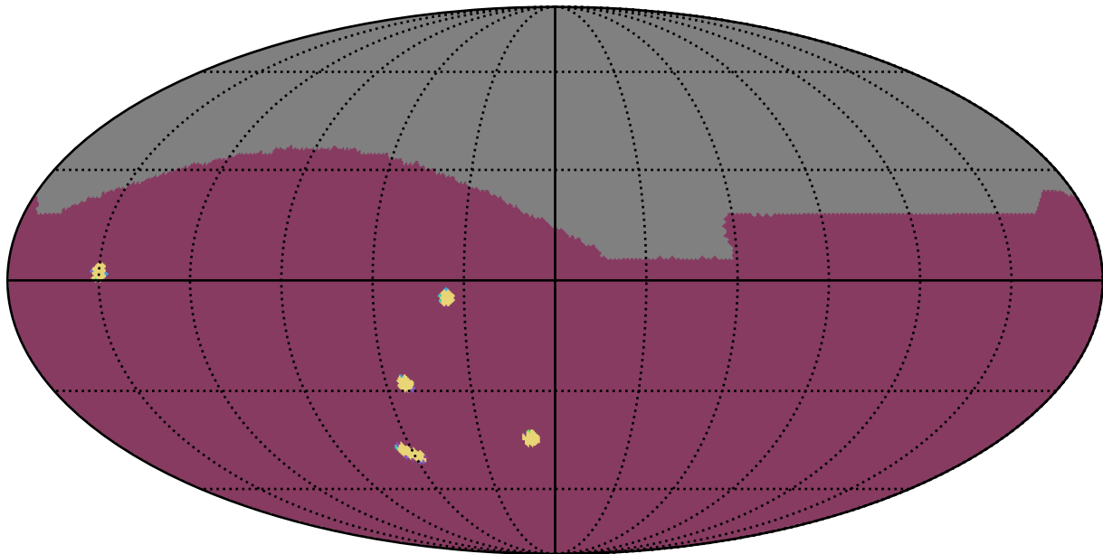
early_u_fpextra2.0_v3.4_10yrs All sky: NumberOfQuickRevisits
