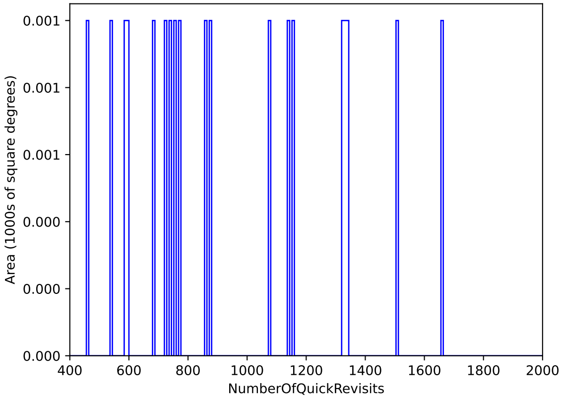
early_u_fpextra2.0_v3.4_10yrs All sky: NumberOfQuickRevisits
