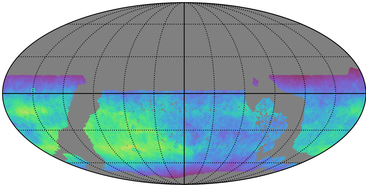
early_u_fpextra2.0_v3.4_10yrs WFD z band: Normalized Teff
