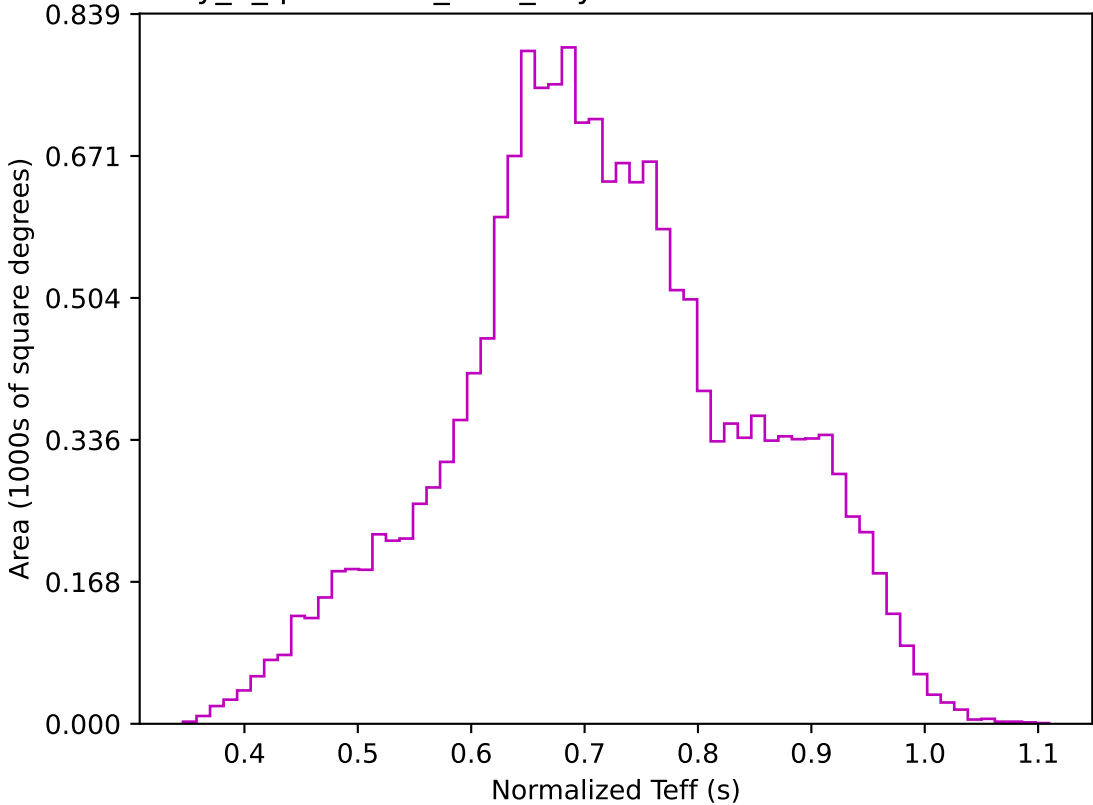
early_u_fpextra2.0_v3.4_10yrs WFD z band: Normalized Teff
