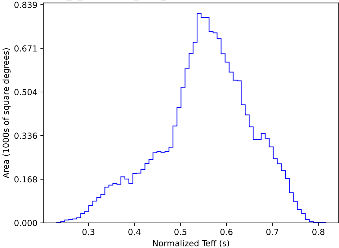
early_u_fpextra2.0_v3.4_10yrs WFD y band: Normalized Teff
