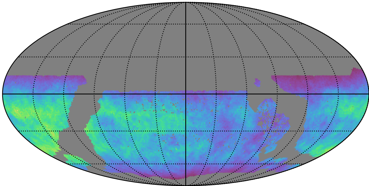
early_u_fpextra2.0_v3.4_10yrs WFD u band: Normalized Teff
