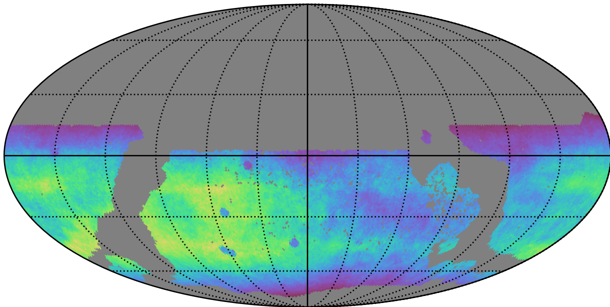
early_u_fpextra2.0_v3.4_10yrs WFD r band: Normalized Teff
