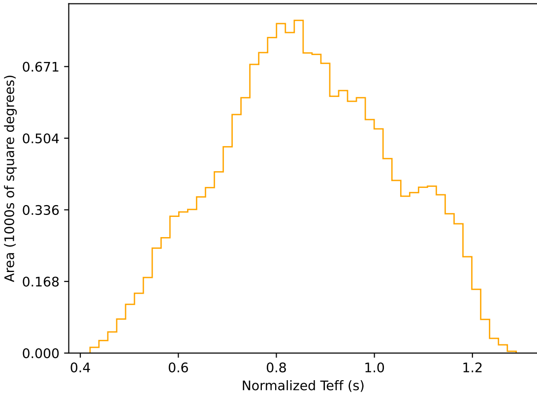
early_u_fpextra2.0_v3.4_10yrs WFD r band: Normalized Teff
