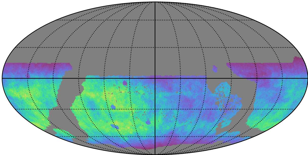
early_u_fpextra2.0_v3.4_10yrs WFD g band: Normalized Teff
