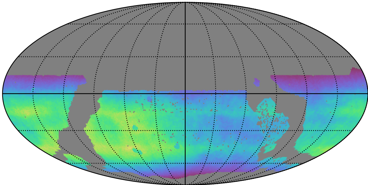
early_u_fpextra2.0_v3.4_10yrs WFD all bands: Normalized Teff
