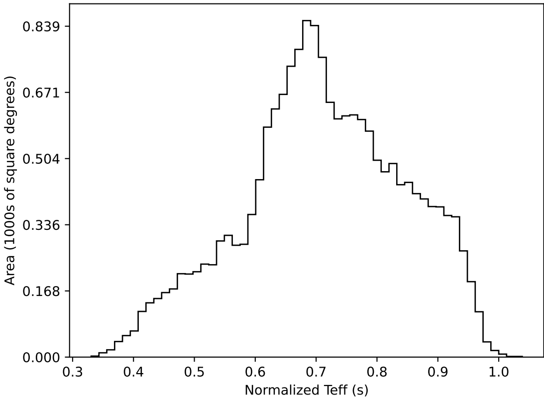
early_u_fpextra2.0_v3.4_10yrs WFD all bands: Normalized Teff
