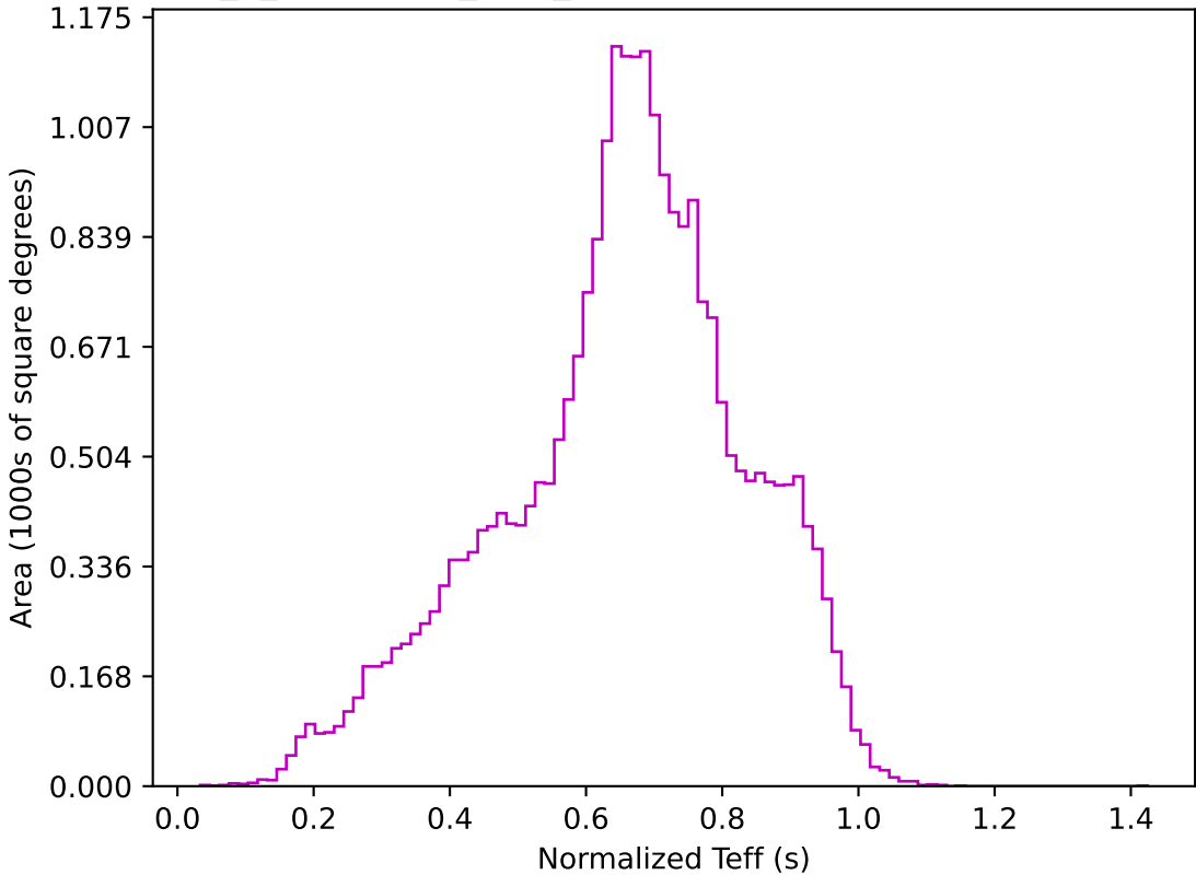
early_u_fpextra2.0_v3.4_10yrs All sky z band: Normalized Teff
