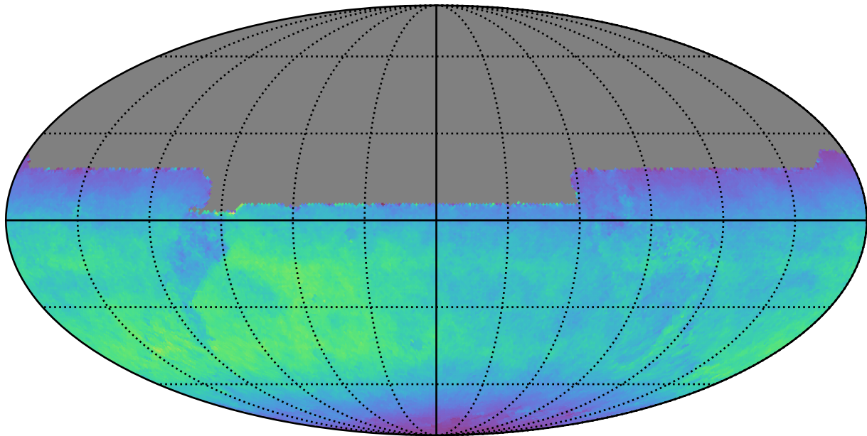
early_u_fpextra2.0_v3.4_10yrs All sky y band: Normalized Teff
