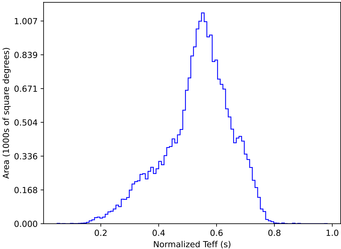
early_u_fpextra2.0_v3.4_10yrs All sky y band: Normalized Teff
