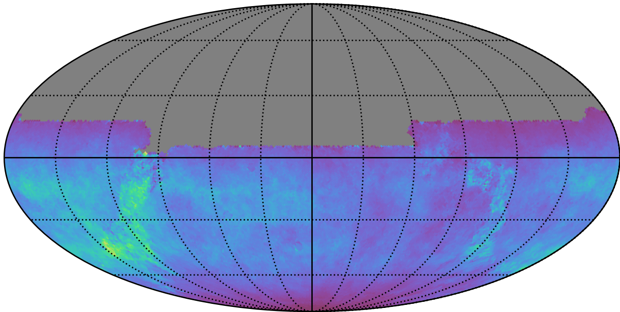
early_u_fpextra2.0_v3.4_10yrs All sky u band: Normalized Teff
