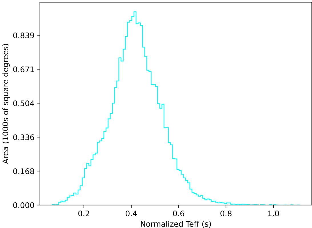
early_u_fpextra2.0_v3.4_10yrs All sky u band: Normalized Teff
