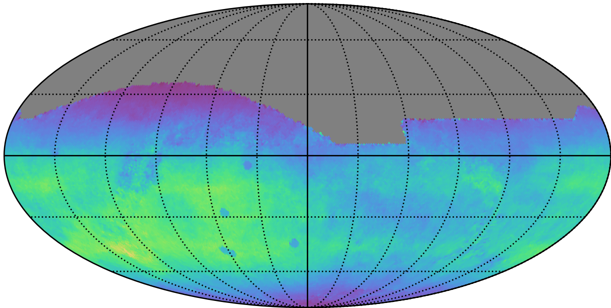
early_u_fpextra2.0_v3.4_10yrs All sky r band: Normalized Teff
