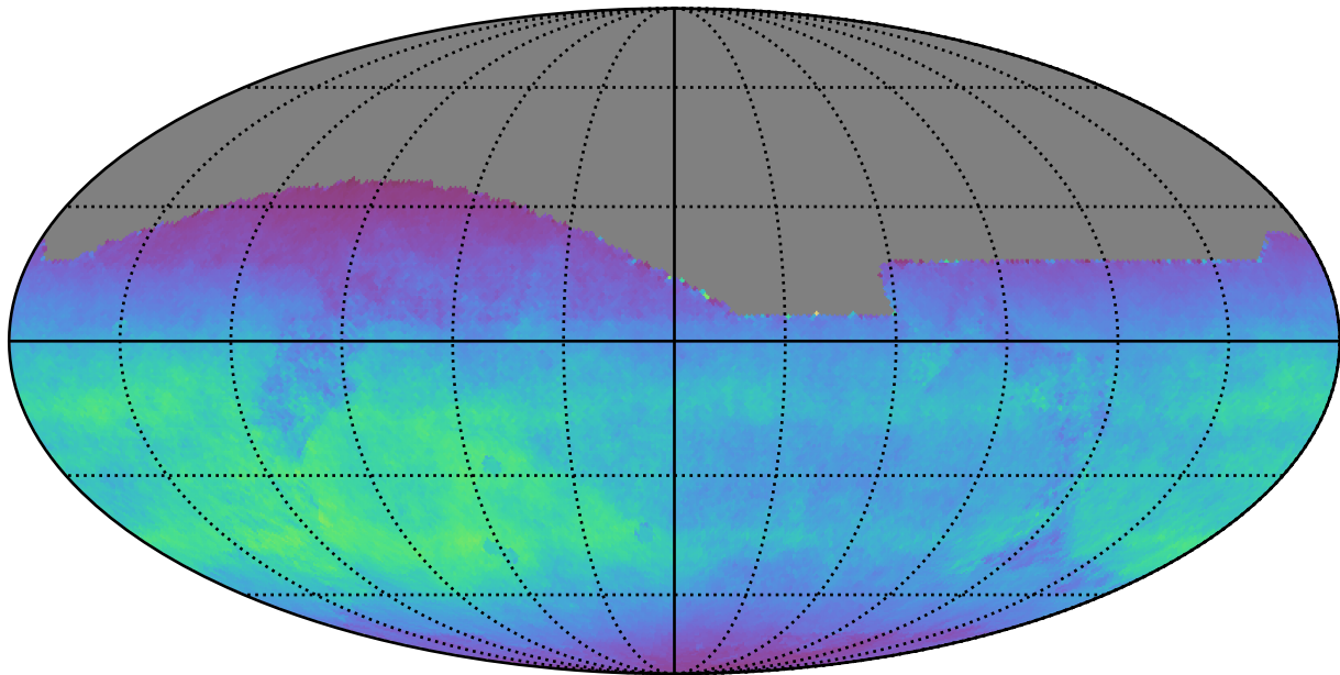
early_u_fpextra2.0_v3.4_10yrs All sky i band: Normalized Teff
