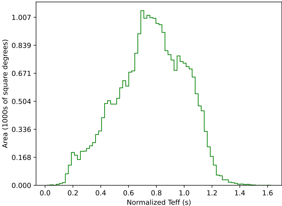
early_u_fpextra2.0_v3.4_10yrs All sky g band: Normalized Teff
