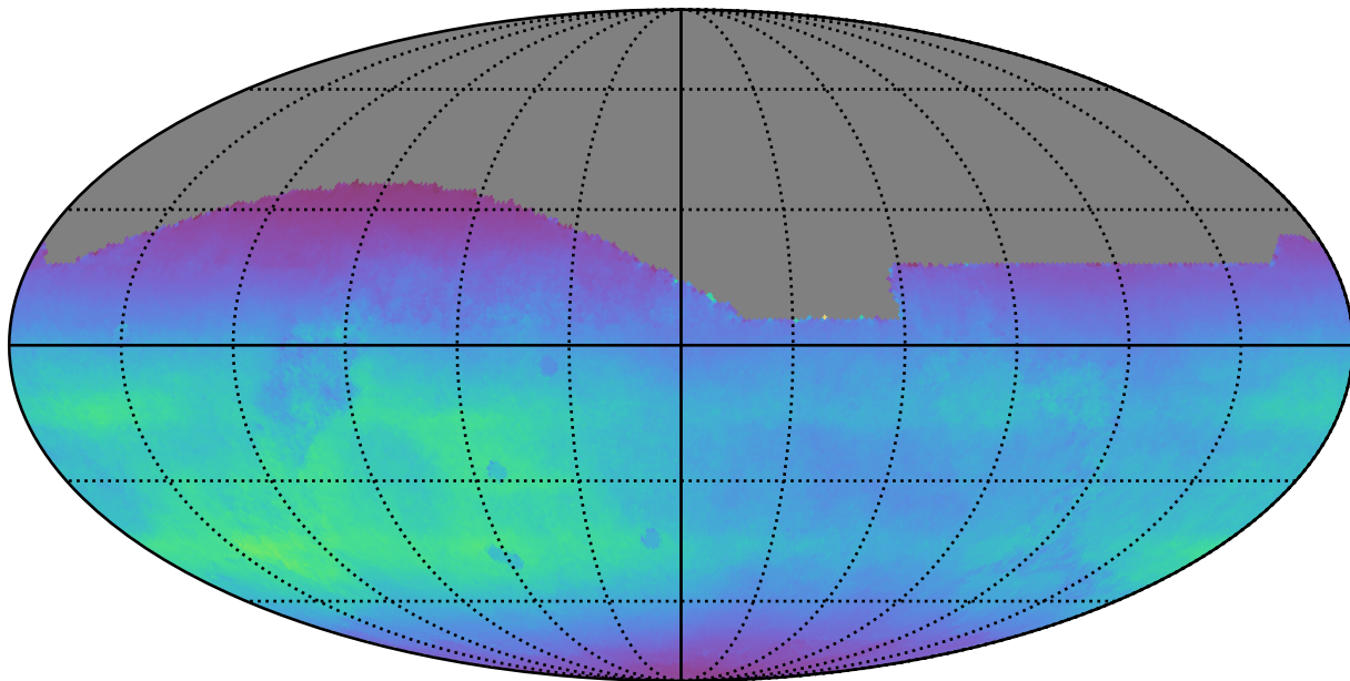
early_u_fpextra2.0_v3.4_10yrs All sky all bands: Normalized Teff
