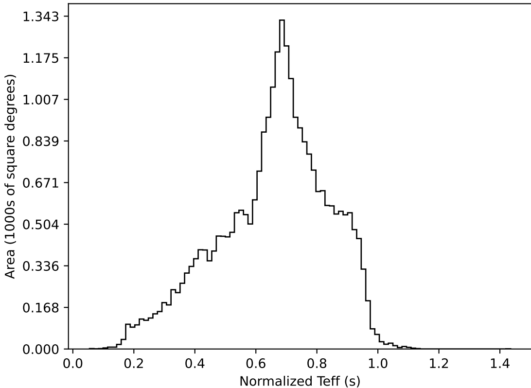
early_u_fpextra2.0_v3.4_10yrs All sky all bands: Normalized Teff
