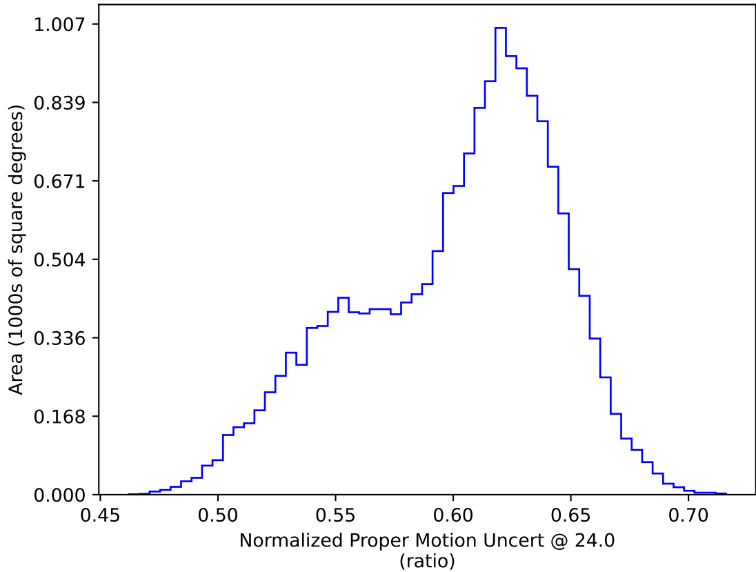
early_u_fpextra2.0_v3.4_10yrs WFD: Normalized Proper Motion Uncert @ 24.0
