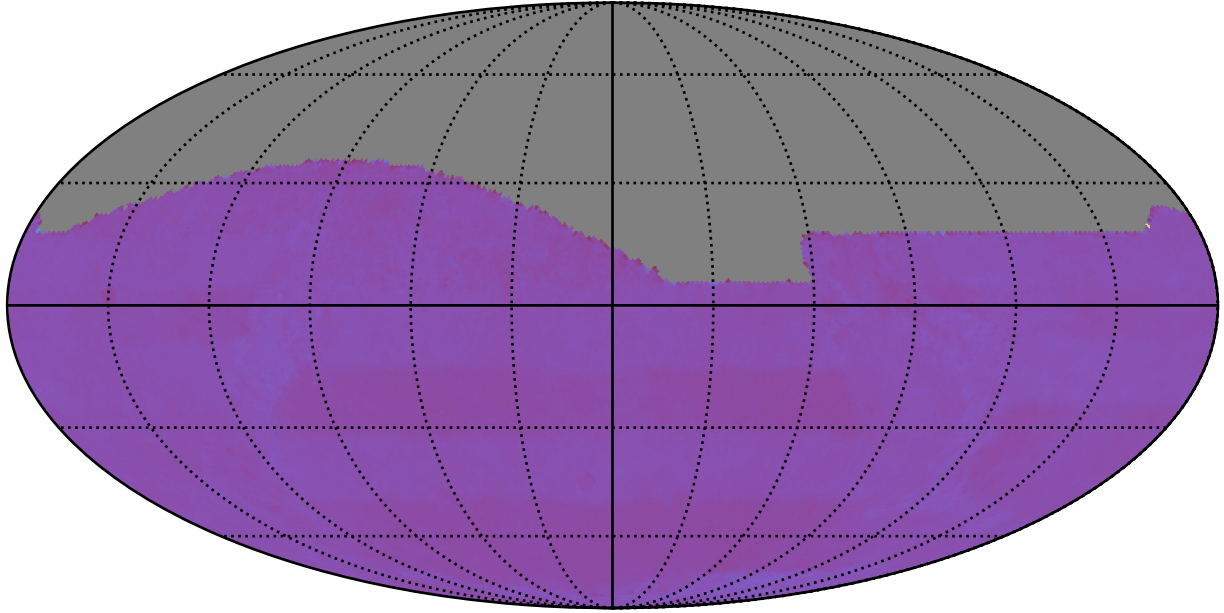
early_u_fpextra2.0_v3.4_10yrs All sky: Normalized Proper Motion Uncert @ 24.0
