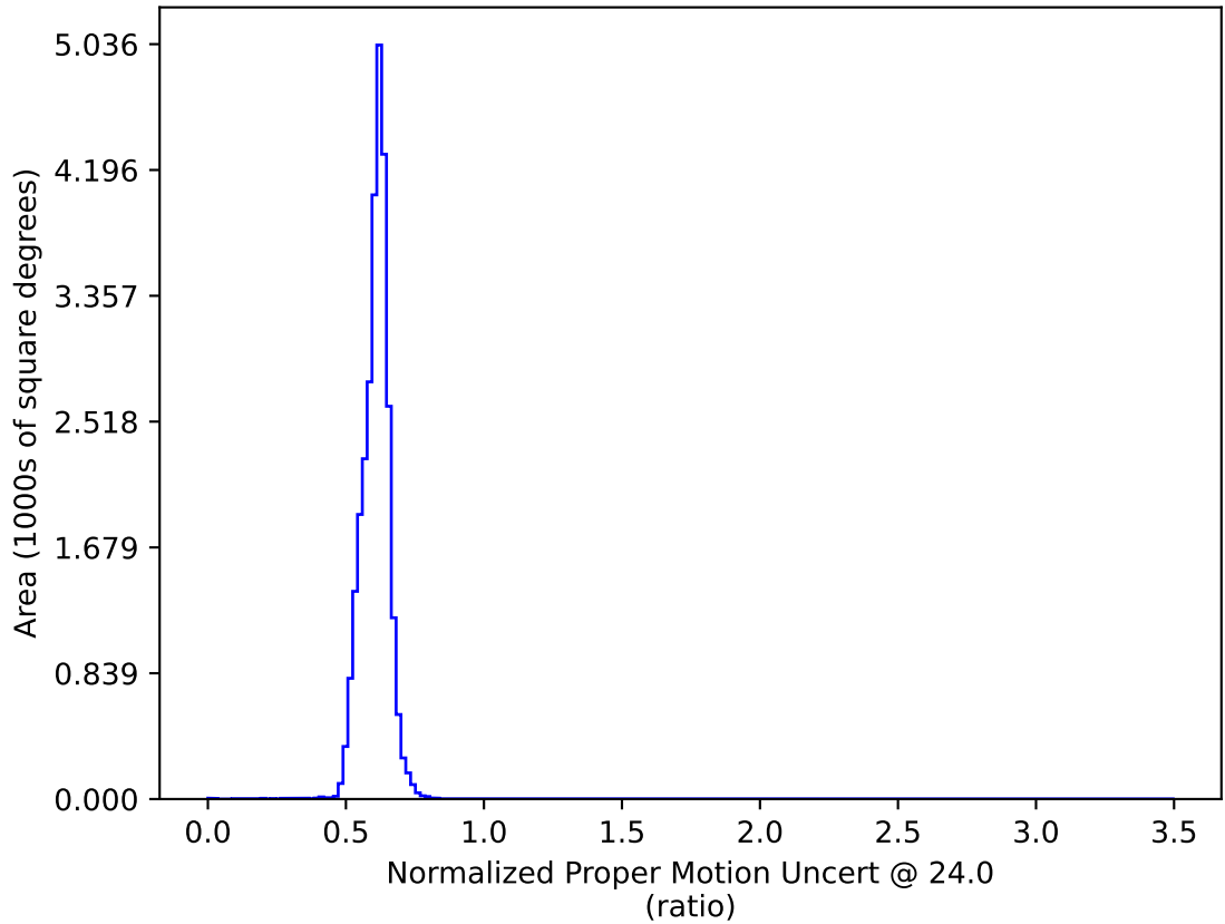
early_u_fpextra2.0_v3.4_10yrs All sky: Normalized Proper Motion Uncert @ 24.0
