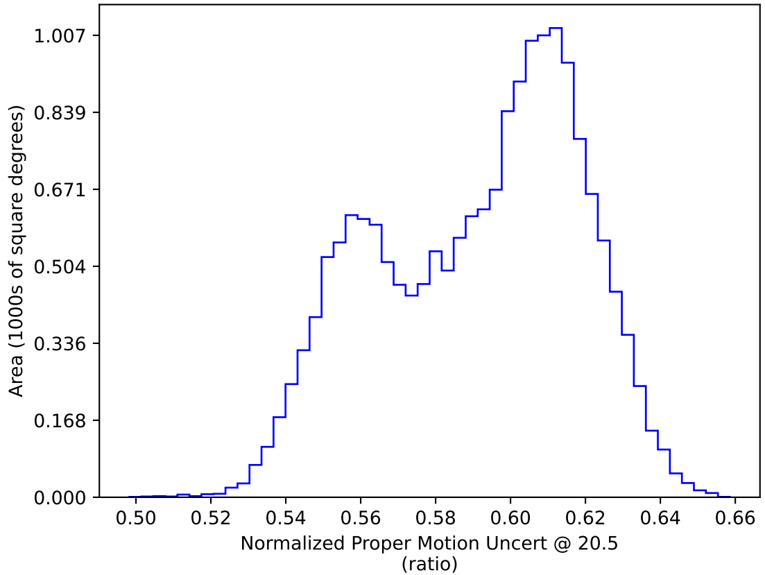
early_u_fpextra2.0_v3.4_10yrs WFD: Normalized Proper Motion Uncert @ 20.5
