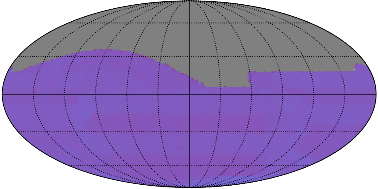
early_u_fpextra2.0_v3.4_10yrs All sky: Normalized Proper Motion Uncert @ 20.5
