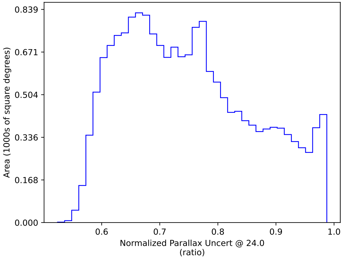
early_u_fpextra2.0_v3.4_10yrs WFD: Normalized Parallax Uncert @ 24.0
