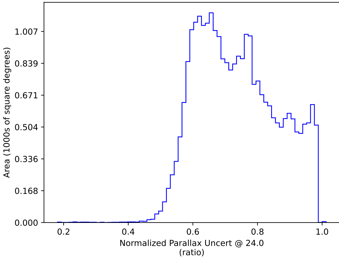
early_u_fpextra2.0_v3.4_10yrs All sky: Normalized Parallax Uncert @ 24.0
