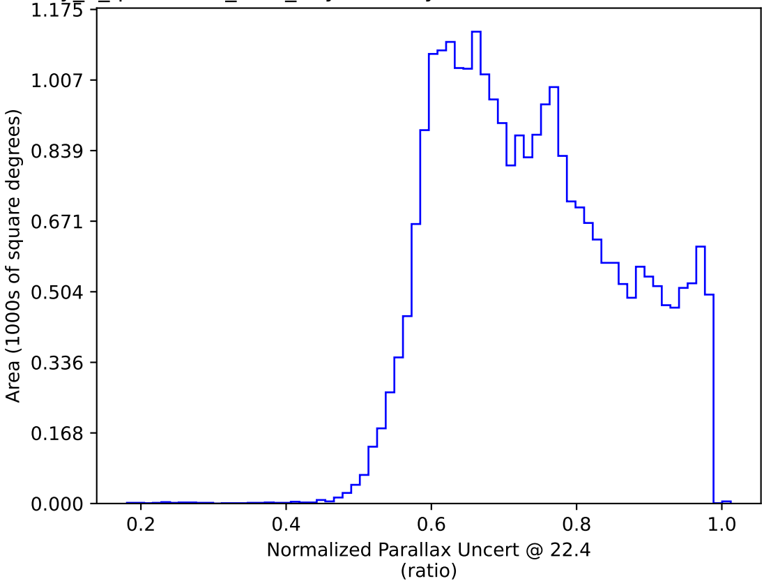
early_u_fpextra2.0_v3.4_10yrs All sky: Normalized Parallax Uncert @ 22.4
