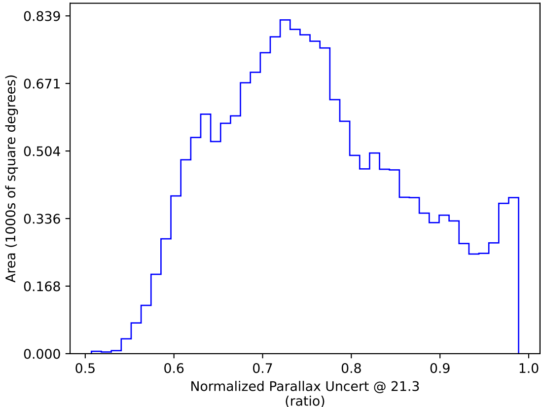
early_u_fpextra2.0_v3.4_10yrs WFD y band only: Normalized Parallax Uncert @ 21.3
