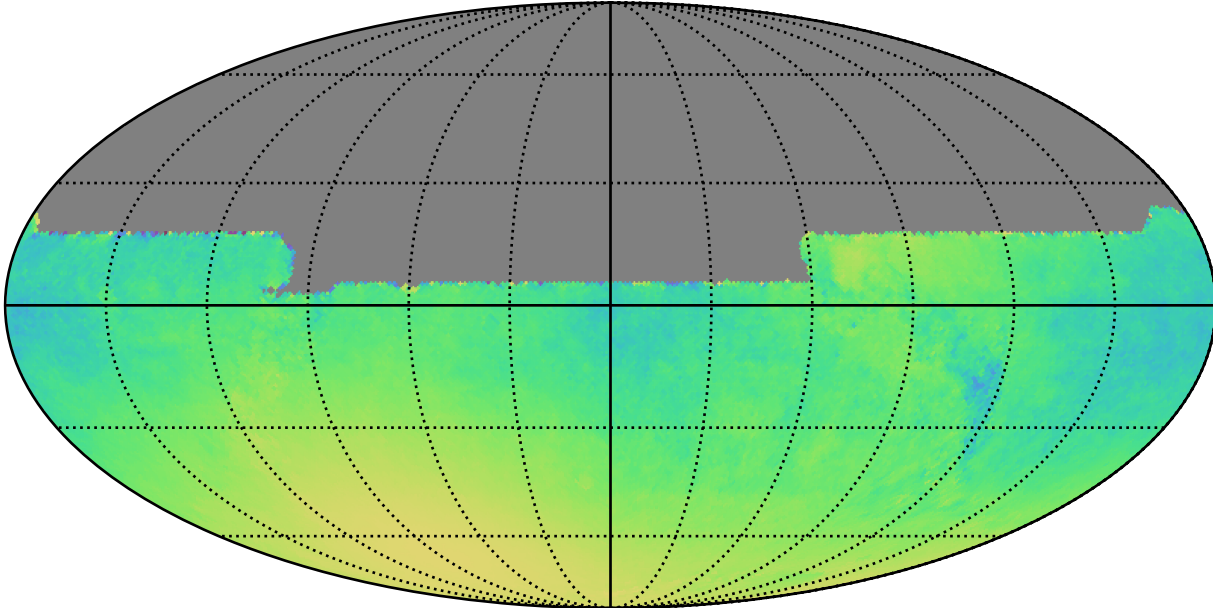
early_u_fpextra2.0_v3.4_10yrs All sky y band only: Normalized Parallax Uncert @ 21.3
