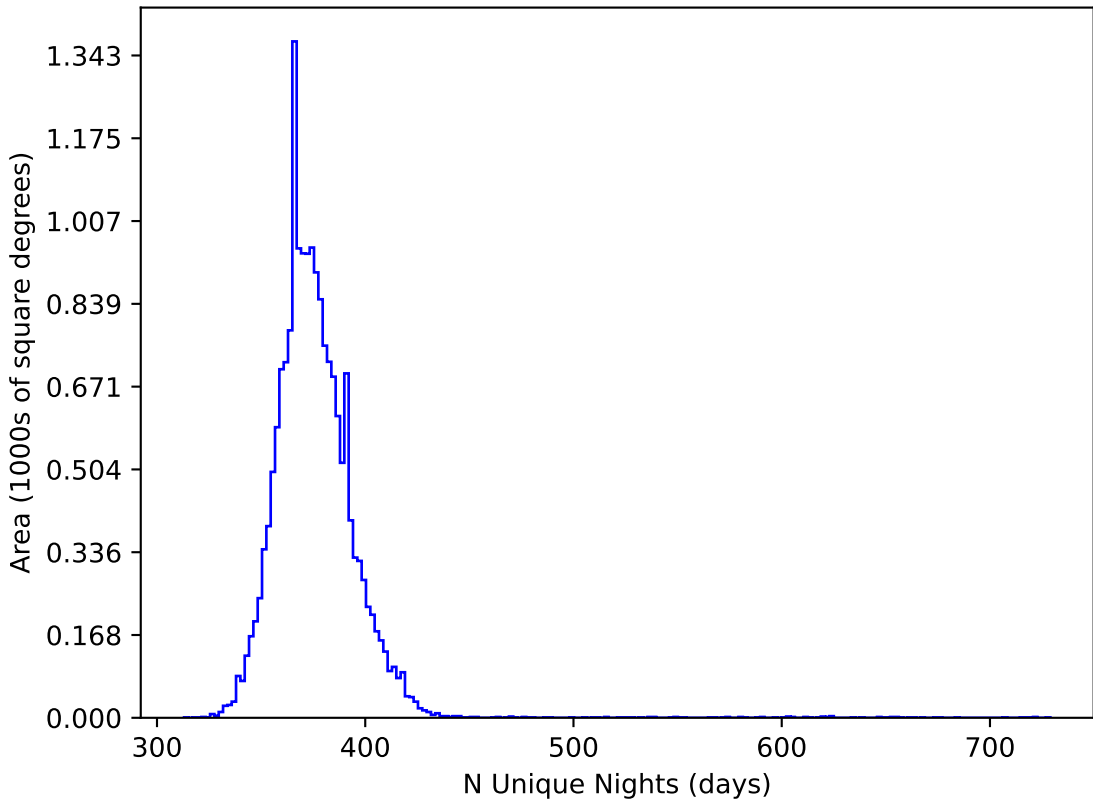
early_u_fpextra2.0_v3.4_10yrs WFD all bands: N Unique Nights
