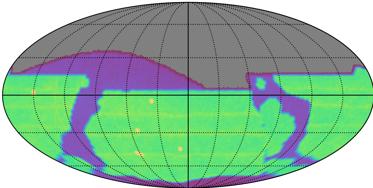
early_u_fpextra2.0_v3.4_10yrs All sky all bands: N Unique Nights
