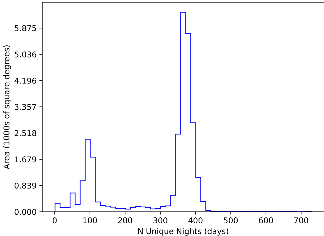
early_u_fpextra2.0_v3.4_10yrs All sky all bands: N Unique Nights
