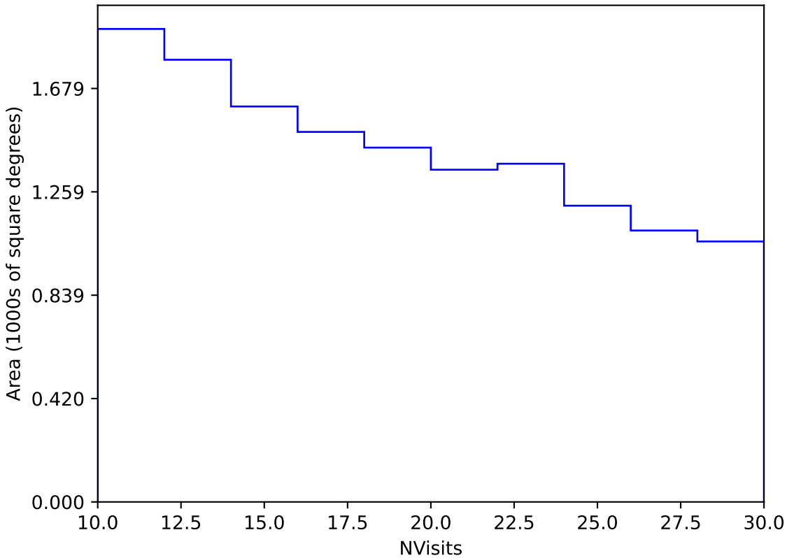
early_u_fpextra2.0_v3.4_10yrs Yr 3-4 y band: NVisits
