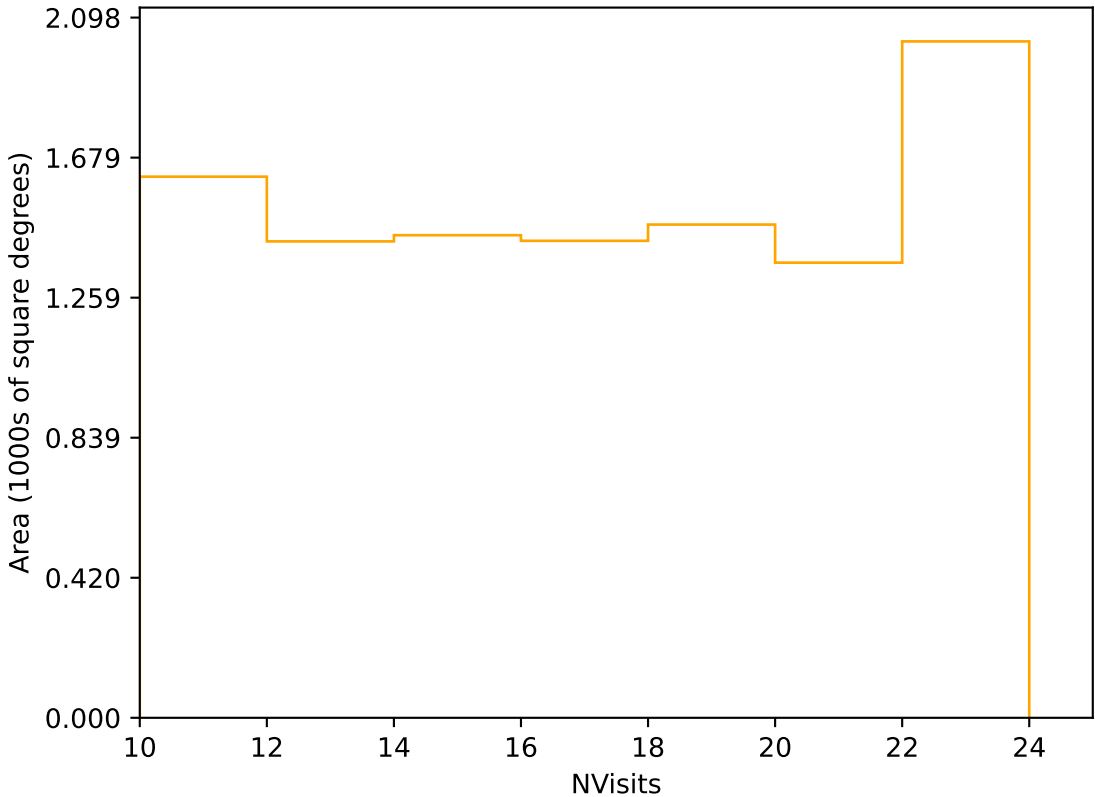
early_u_fpextra2.0_v3.4_10yrs Yr 3-4 r band: NVisits
