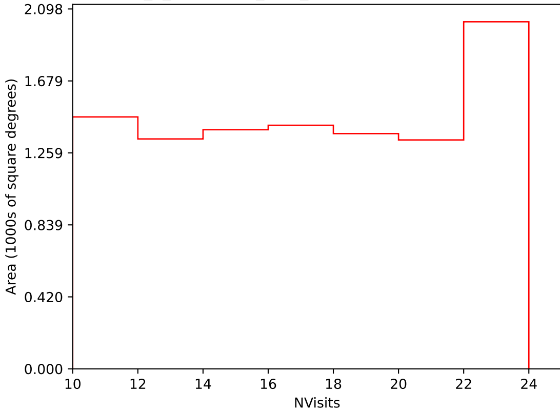
early_u_fpextra2.0_v3.4_10yrs Yr 3-4 i band: NVisits
