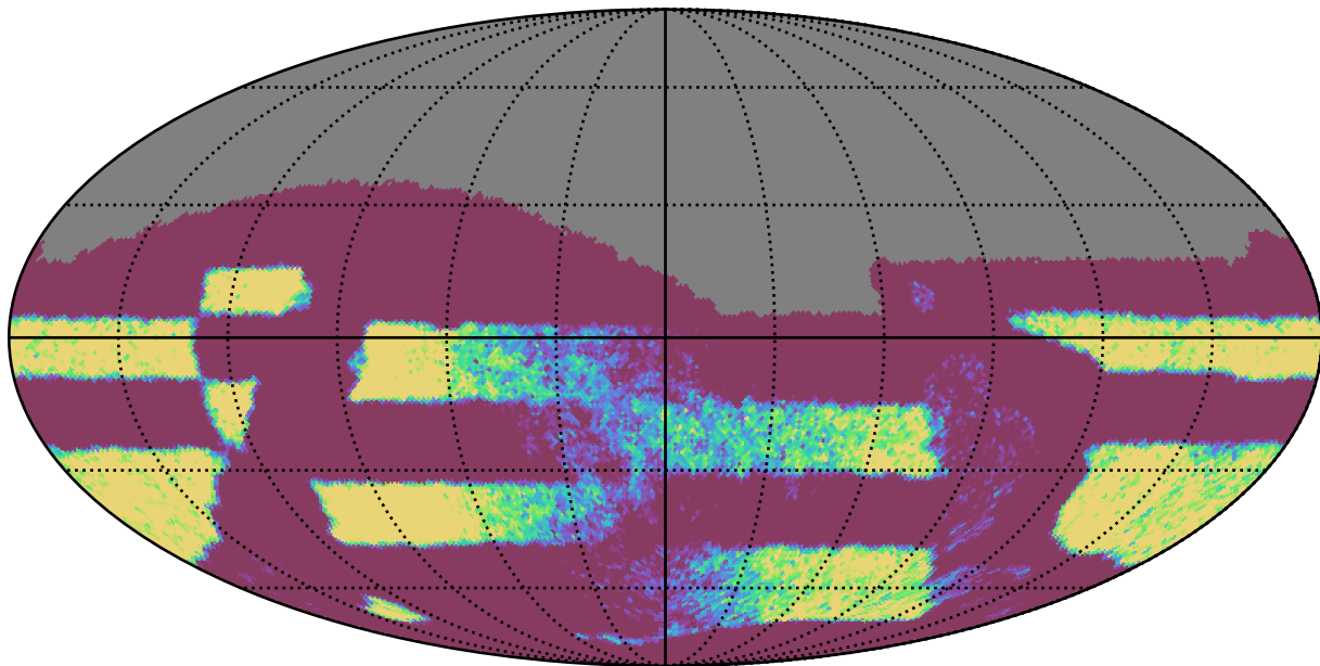
early_u_fpextra2.0_v3.4_10yrs Yr 3-4 all bands: NVisits
