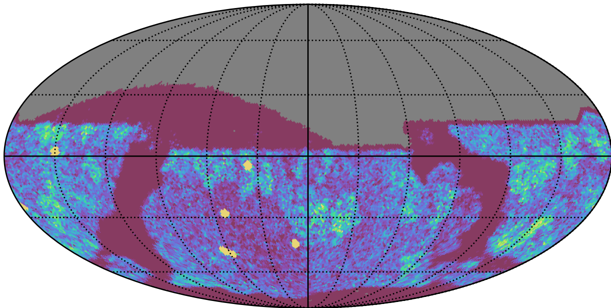
early_u_fpextra2.0_v3.4_10yrs Yr 1 z band: NVisits
