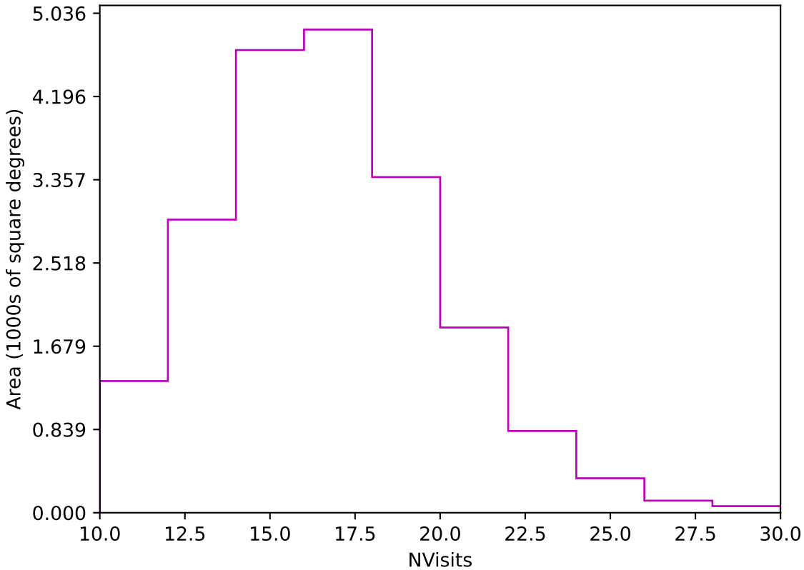
early_u_fpextra2.0_v3.4_10yrs Yr 1 z band: NVisits
